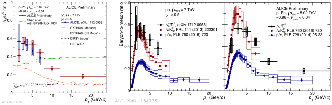
Fig. 1. The \Lambda_c^+/D^0 ratio in pp collisions at \sqrt{s} = 7 TeV and in p-Pb collisions at \sqrt{s_{NN}} = 5.02 TeV, compared with model predictions (left) and \Lambda_c^+/K_s^0 , p/\pi ratios in pp (middle) and p-Pb (right) collisions.
