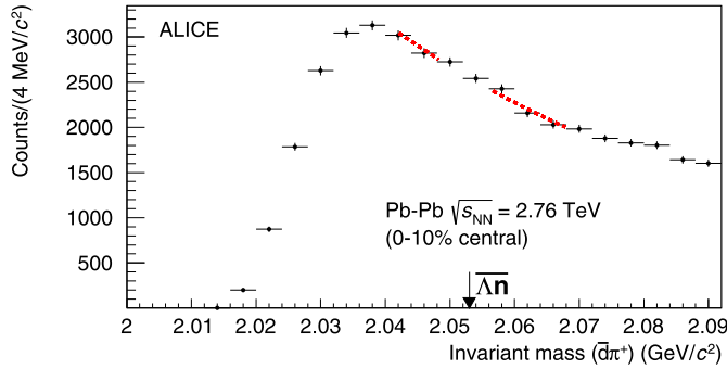
Fig. 2. Invariant mass distribution for \bar{d}\pi^+ for the Pb–Pb data corresponding to 19.3 \times 10^6 central events. The arrow indicates the sum of the mass of the constituents ( \bar{\Lambda}n ) of the assumed bound state. A signal for the bound state is expected in the region below this sum. The dashed line represents an exponential fit outside the expected signal region to estimate the background.
