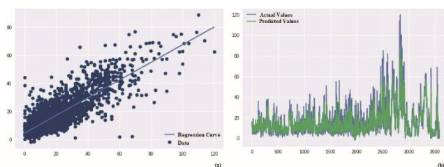
Figure 6. (a) Regression curve of actual (y-axis) and predicted (x-axis) values for two-hour prediction (b) comparison of actual and predicted results (y-axis) with respect to time in seconds (x-axis) for two-hour prediction
