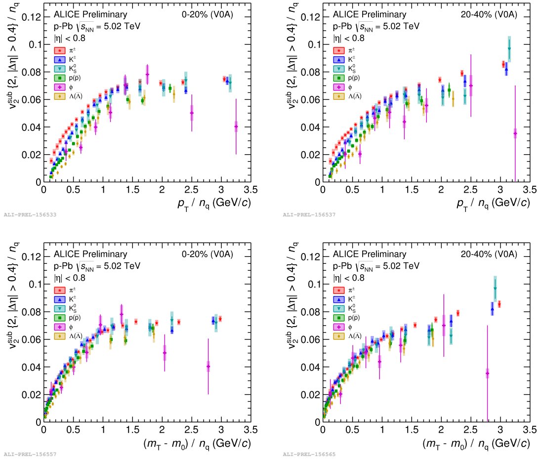
Fig. 2. Test of scaling properties of v_2 coefficients. Upper row: both v_2^{\text{sub}} and p_T are scaled by number of constituent quarks n_q (NCQ scaling). Bottom row: transverse kinetic energy ( \text{KE}_T ) scaling, where rest mass m_0 of individual species is subtracted from m_T .
