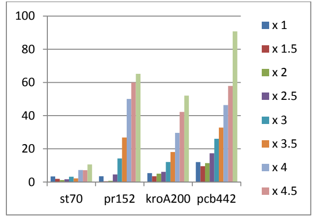
Figure 2 Best distance results of running proposed algorithm on four TSPLIB TSP benchmark instances with some defined fixed number of neurons in multiples of number of cities
