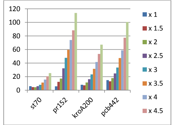
Figure 1. Average distance results of running proposed algorithm on four TSPLIB TSP benchmark instances with some defined fixed number of neurons in multiples of number of cities 1
